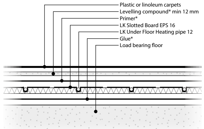
LK EPS 16 glued on load bearing floor in wet areas. Surface layer plastic or linoleum carpets
